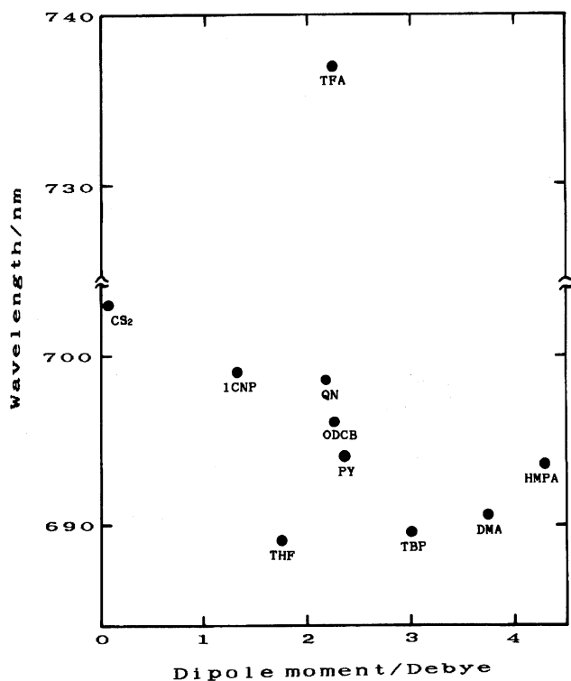
Fig. 10. Plot of the Q_x band wavelength of a solution containing H 2 pc vs. the dipole moment of the solvent. A single peak was observed in TFA.
