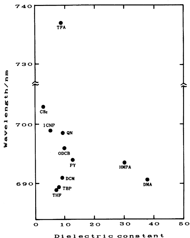
Fig. 9. Plot of the Q_x band wavelength of a solution containing H 2 pc vs. the dielectric constant of the solvent.
