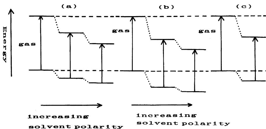
Fig. 6. Schematic energy diagram of solvent effects on the electronic transition of TiOpc in solvents. (a) in dipolar solvent, (b) in coordinating solvent, (c) in CS 2 .
